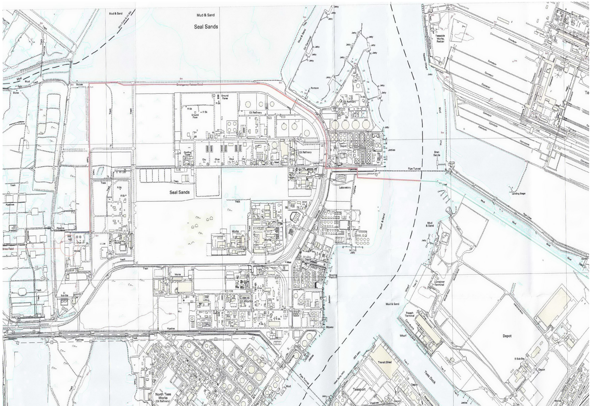
Proposed Pipeline Route (Stockton Borough Council in Red) from River Tees to Teesside Gas Processing Plant.
